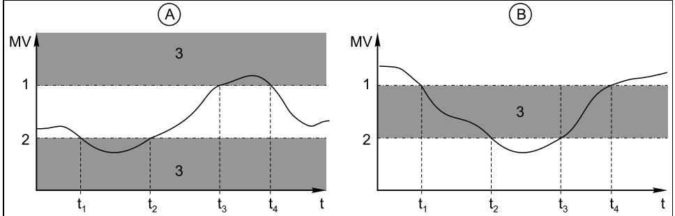
Abb. 10: Monitoring outside (A) and within (B) a range (without hysteresis and switch-on delay)
