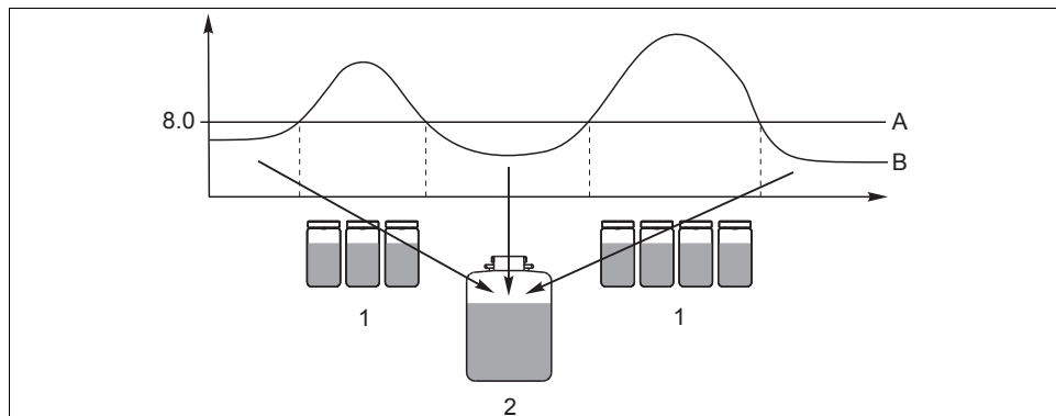
Abb. 8: Event-controlled sampling
