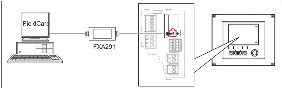
Fig. 15: Connection overview
