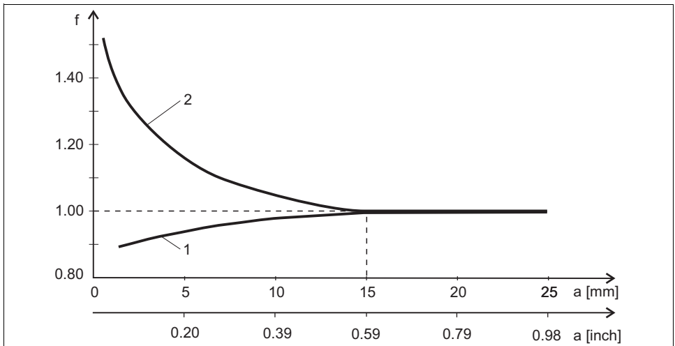
Fig. 18: Relation between the installation factor f and the wall distance
