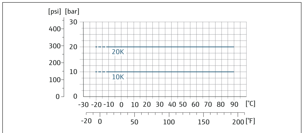
18 过程连接材质: 不锈钢 (-20°C (-4°F)) ; 碳钢 (-10°C (14°F))
